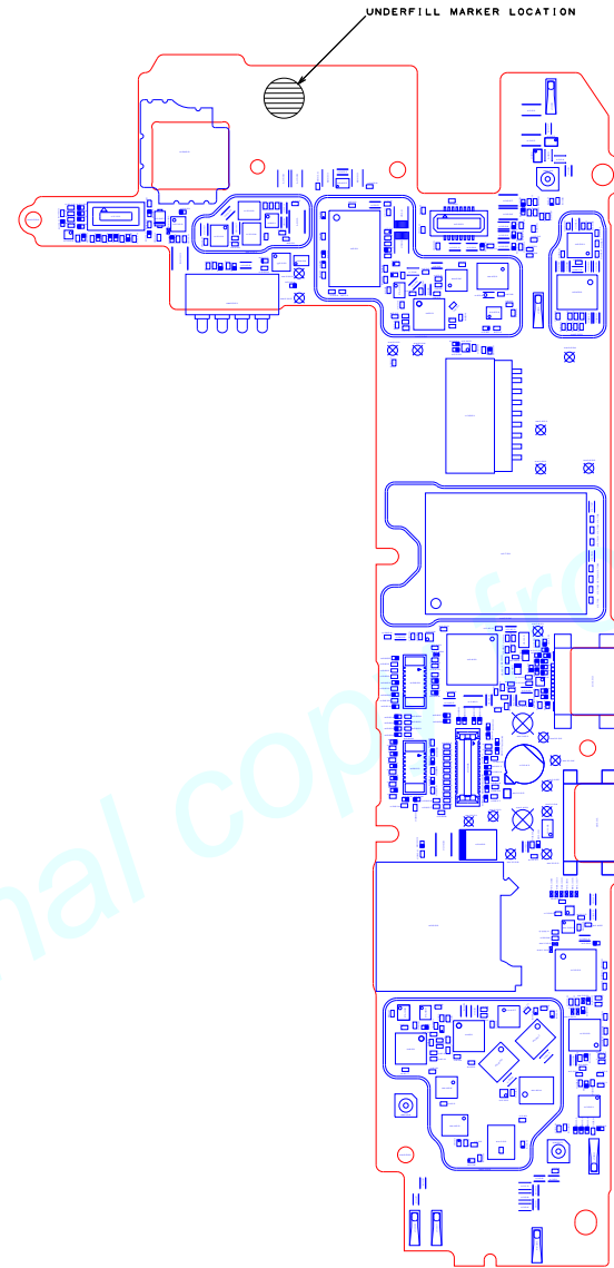
PCB ASSEMBLY VIEWED FROM SECONDARY SIDE (SIDE B)
