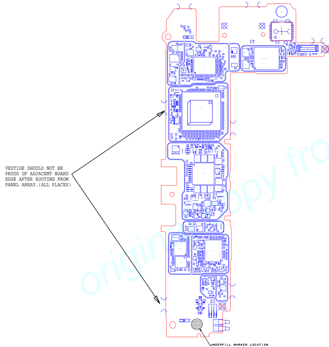
PCB ASSEMBLY VIEWED FROM PRIMARY SIDE (SIDE A)
